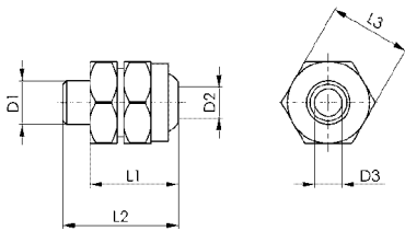
Order no. 17699: ball joint
