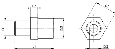
Order no. 17673: adapter
