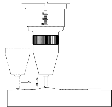
Fig. 1 Uneven workpiece surface
