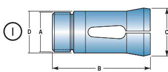
Internal stop thread is 1.687" x 20 RH.
