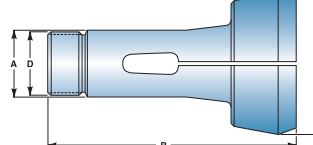
Internal stop thread is 1.687" x 20 RH. An extra depth closer is required
